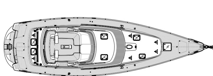
DECK LAYOUT
