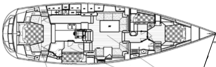
INTERIOR LAYOUT
